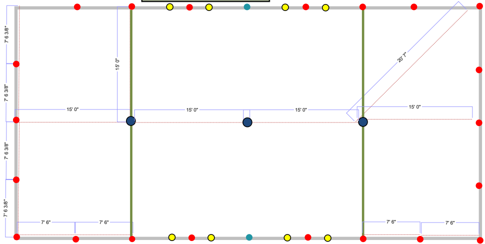
30' x 60' Pole Tent Standard & Wind - Pole placement
